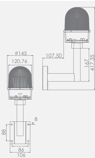
Obstruction Lights
