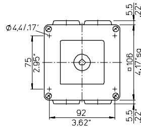
For switch type A11, A14, CA40, CA50, CA63
